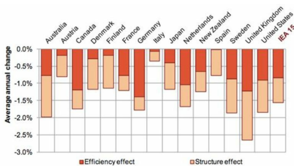
Figure 8: Changes in aggregate intensities of 15 member IEA countries, decomposed into structure and efficiency effects, 1990-2010. Source: IEA Energy Efficiency Market Report 2013, Figure 3.10
