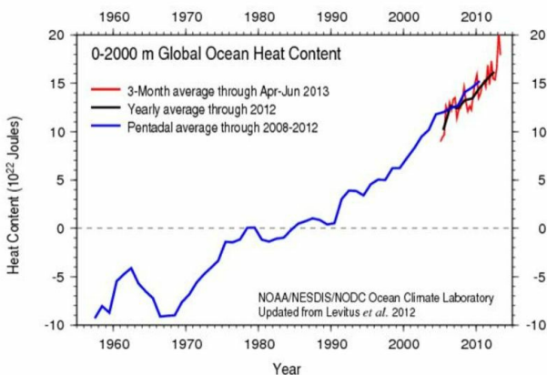
Figure 5: Five Decades of Global Ocean Heat Content, 0 to 2000 meters. Source.
