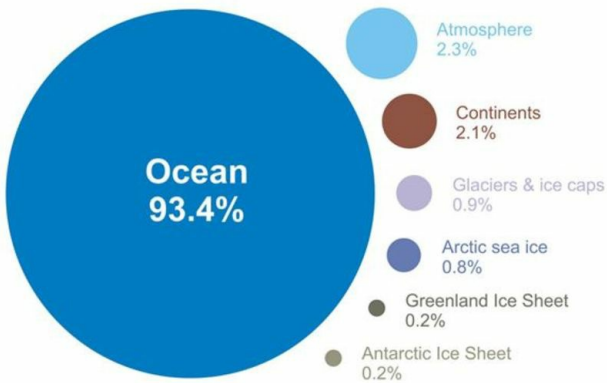
Figure 3: Heat Absorption By Terrestrial Climate Systems. Source.
