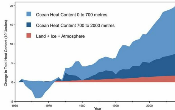
Figure 4: Trends in Climate System Heat Absorption, 1960-2008. Source.
