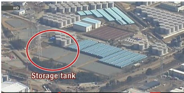
Leaking storage tank and TEPCO attempts to contain contaminated water at Fukushima Daiichi (NHK)
