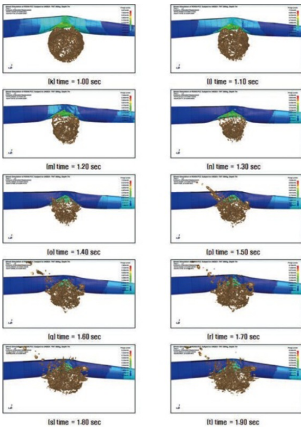
Figure 6-26 and Figure 6-23, however, created the illusion that the simulation showed: the severance of the ship in the middle.
